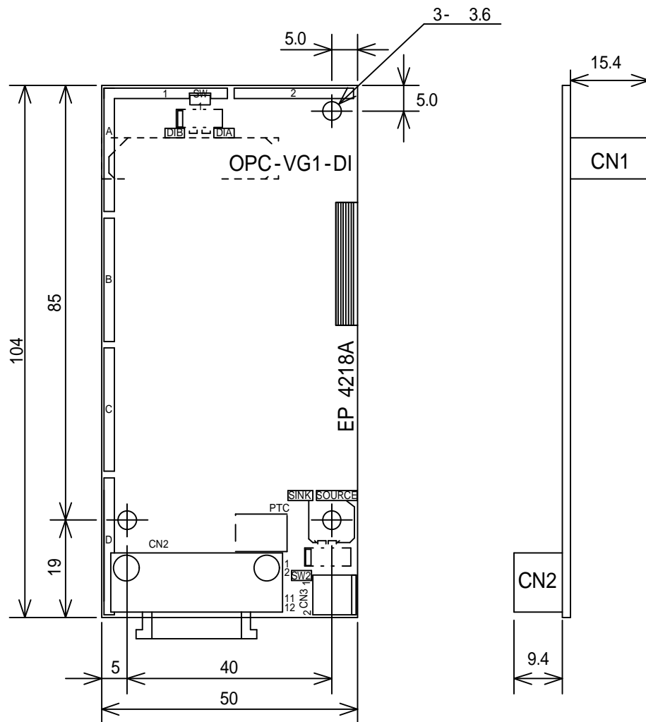
Figure 1.2-1 External Appearance
