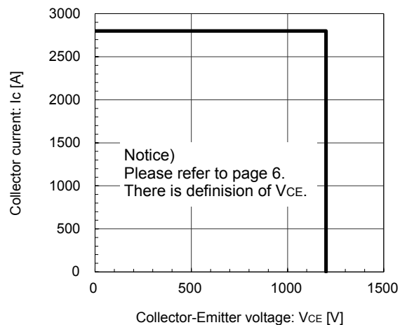
Reverse bias safe operating area (max.) +V_{GE}=15V, -V_{GE}=15V, R_G=1.0\Omega, T_j=150^\circ C
