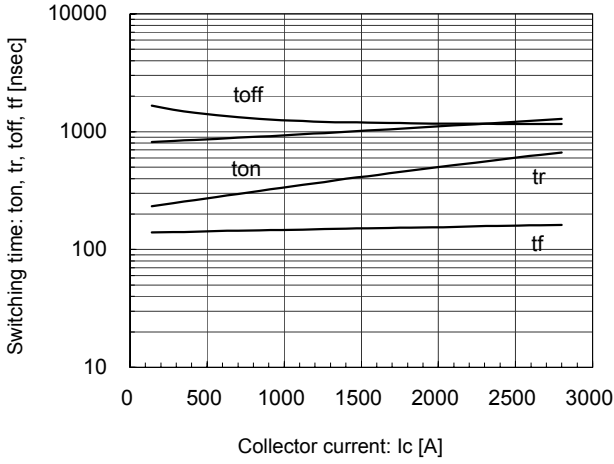
Switching time vs. Collector current (typ.) V_{CC}=600V, V_{GE}=\pm 15V, R_G=1.0\Omega, T_j=25^\circ C
