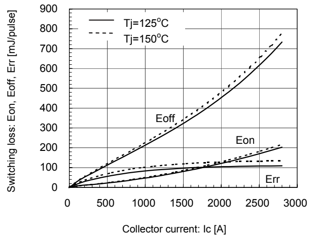
Switching loss vs. Collector current (typ.) V_{CC}=600V, V_{GE}=\pm 15V, R_G=1.0\Omega, T_j=125^\circ C, 150^\circ C
