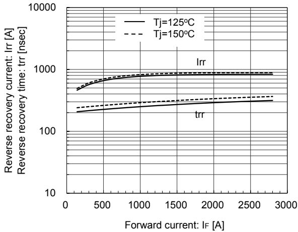
Reverse Recovery Characteristics (typ.) V CC =600V, V GE =±15V, R G =1.0Ω, T j =125°C, 150°C
