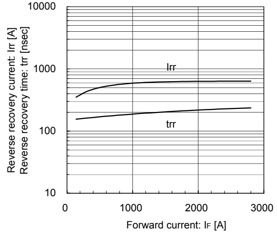
Reverse Recovery Characteristics (typ.) V CC =600V, V GE =±15V, R G =1.0Ω, T j =25°C
