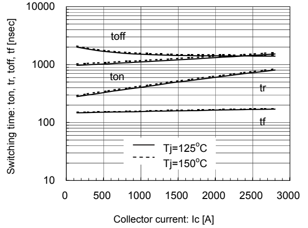
Switching time vs. Collector current (typ.) V_{CC}=600V, V_{GE}=\pm 15V, R_G=1.0\Omega, T_j=125^\circ C, 150^\circ C
